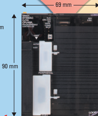
Loop-control CPU Unit
