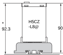
P2CF-08(-E) (order separately) Front Connecting Socket
